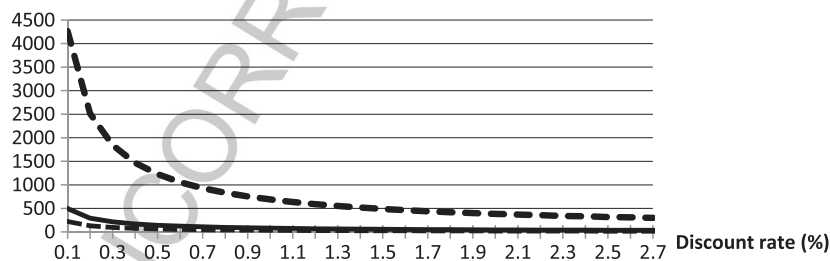
f0075 Fig. 14 Optimal tax rates in current dollars per ton of emitted fossil carbon vs yearly subjective discount rate.
