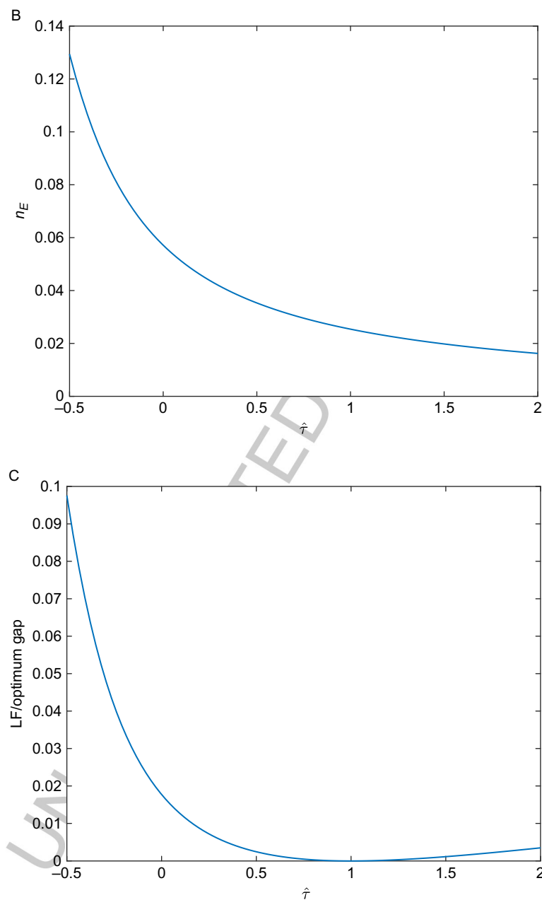
f0060 Fig. 11—cont'd (B) Labor in coal sector. (C) Output gap.
