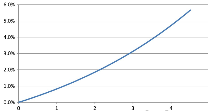
Fig. 10 Damage function using T(S) = 3 \frac{\ln S - \ln S_0}{\ln 2} and D(T(S)) = 1 - e^{-\gamma(T(S))} .
