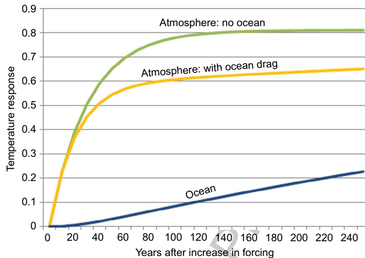
Fig. 6 Increase in atmospheric and ocean temperatures after a permanent forcing of 1W/m^2 .
