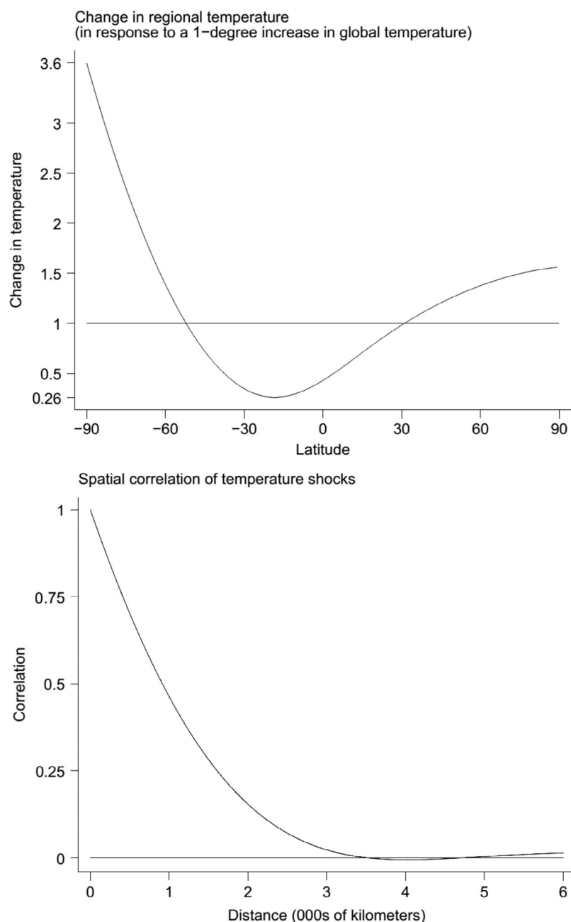
f0040 Fig. 7 Statistical downscaling: regional climate responses to global temperature.
