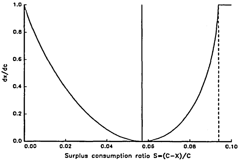
FIG. 1.—a, Sensitivity function \lambda(s) . b, Implied sensitivity of habit x to contemporaneous consumption. The vertical solid line in this and subsequent figures shows the steady-state surplus consumption ratio \bar{S} . The dashed vertical line shows the maximum surplus consumption ratio S_{\max} .
