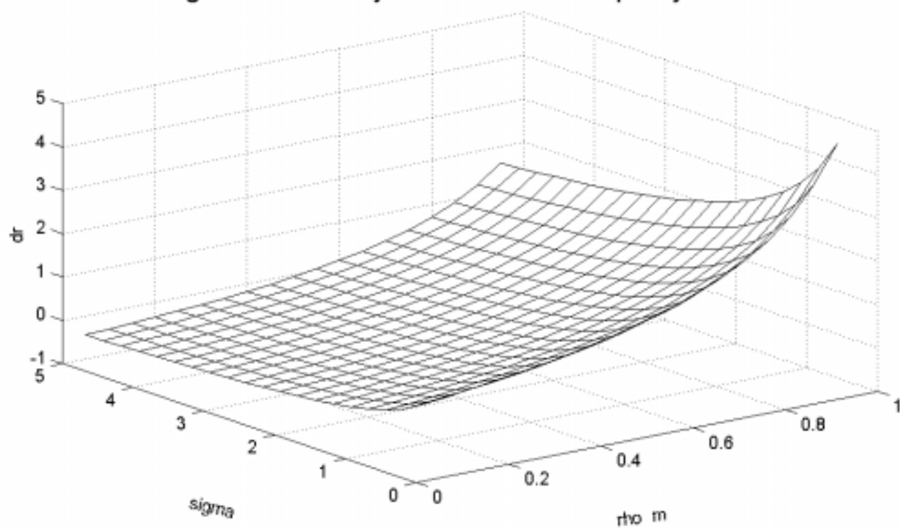
Figure 4: Monetary Shocks and the Liquidity Effect
