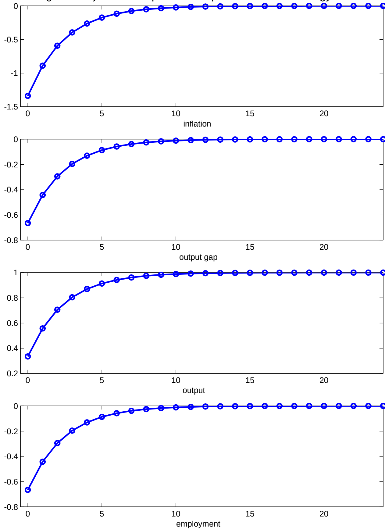
Figure 5: Dynamic Responses Responses to a Technology Shock
