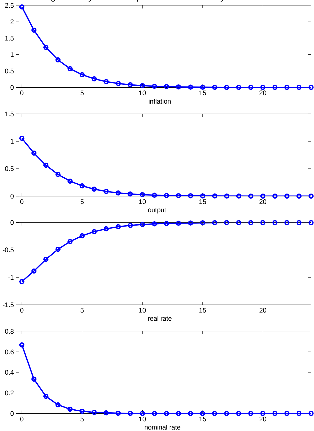
Figure 3: Dynamic Responses to a Monetary Shock
