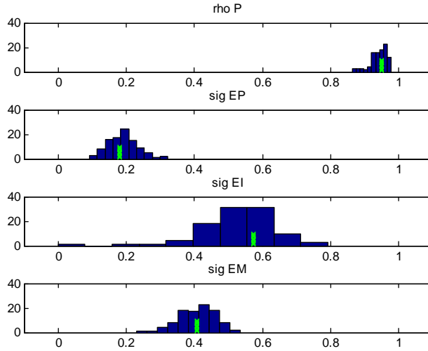
Figure 11: Estimation on simulated data: PIM on PIM high
